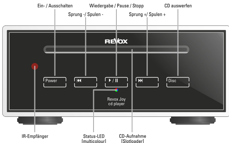
Frontansicht cd player
