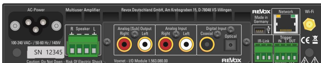
Fig.: M30 with installed I/O module
